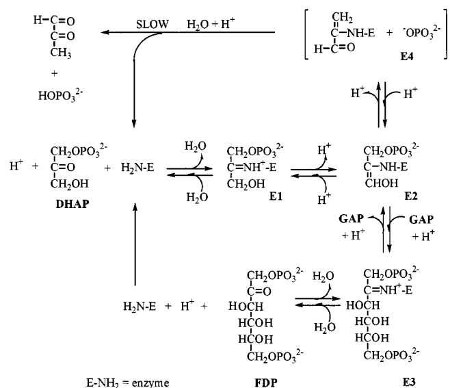
Scheme 1. Reaction catalyzed by aldolase and mechanistic pathway
