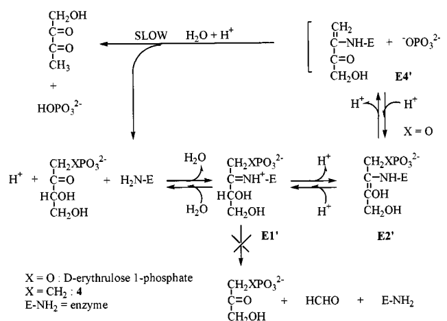
Scheme 3. Proposed mechanism for aldolase inhibition by D-erythrulose 1-phosphate and 4
