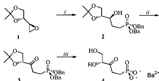
Scheme 2. Synthetic scheme for the synthesis of phosphonate 4 : (i) (\text{BnO})_2\text{P}(\text{O})\text{CH}_3 , \text{BuLi} , \text{Et}_2\text{O}\cdot\text{BF}_3 , THF, -70^\circ\text{C} , 63%; (ii) DCC, pyridine/DMSO, \text{CF}_3\text{CO}_2\text{H} , benzene, 84%; (iii) a) \text{H}_2 , Pd/C, \text{MeOH}/\text{H}_2\text{O} , b) \text{Ba}(\text{OH})_2 , 90%
